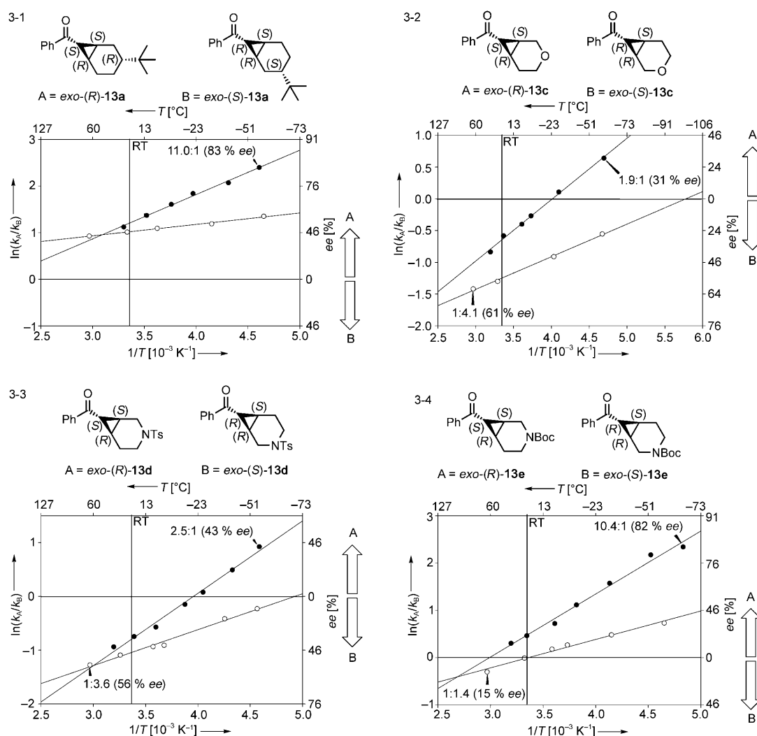
Figure 3. Eyring plots of (R) - 12 \rightarrow exo - 13 : \bullet = \text{CH}_2\text{Cl}_2 , \circ = \text{MeOH} .
